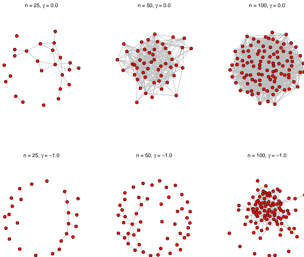
Figure 1: Example Networks
